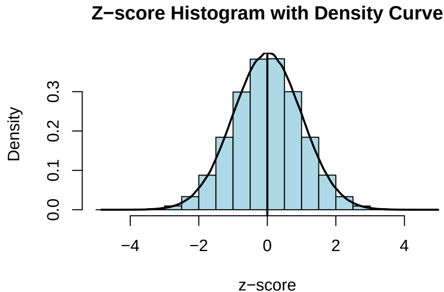
Figure 4.5: The same histogram with the density curve laid over it. dnorm() draws that curve; pnorm() measures the area underneath it.
