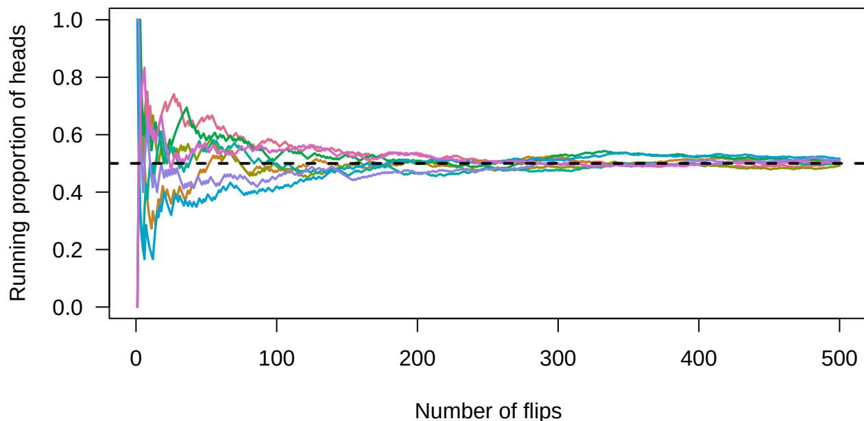
Figure 3.2: The running proportion of heads in eight fair-coin experiments. Early estimates stagger around; with more flips, they become more stable around .50.
