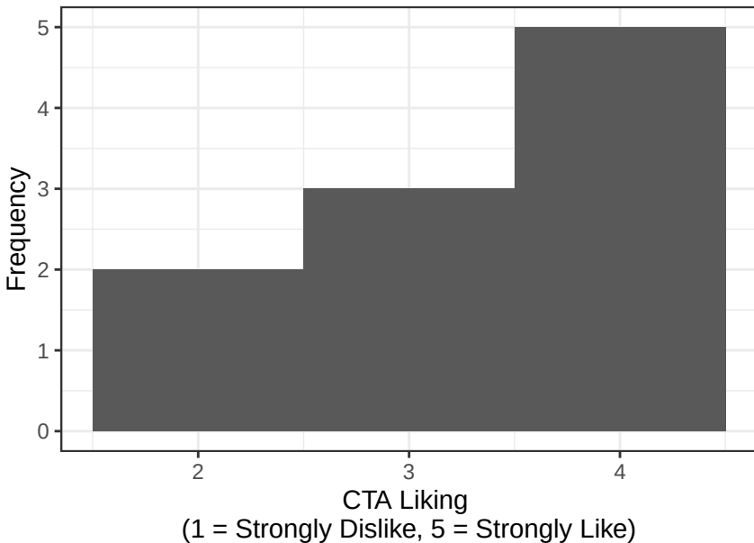
Sample Distribution 2
