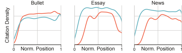
Figure 4: Relative density of citations over normalized text position per style and origin (■ LLM, ■ Human).
