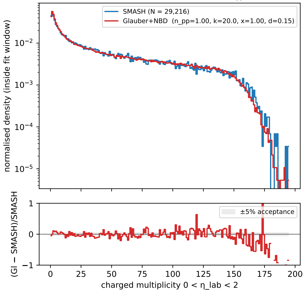
Glauber NBD fit at \sqrt{s_{NN}} = 3.2 GeV \chi^2 = 0.01
