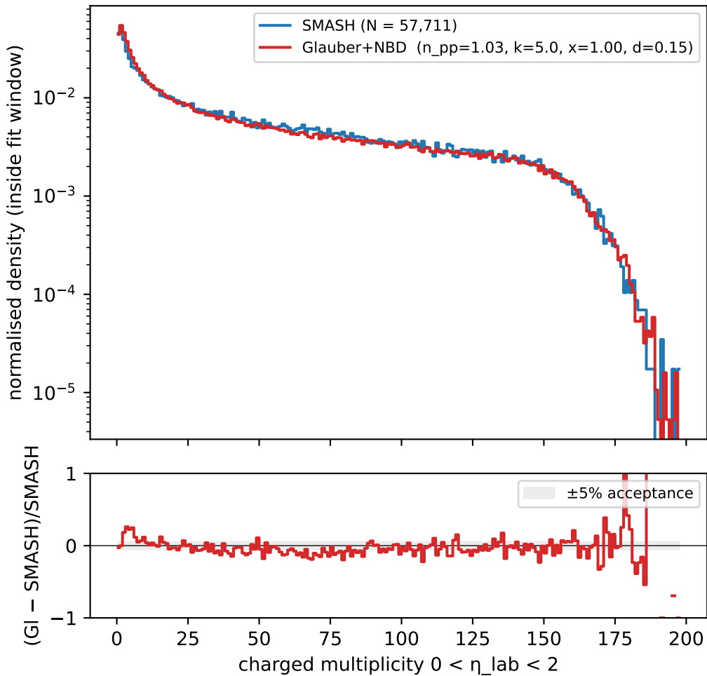
Glauber NBD fit at \sqrt{s_{NN}} = 3.9 GeV \chi^2 = 0.011
