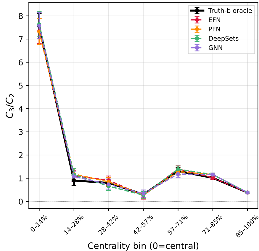
Net-proton cumulant ratios — Au+Au \sqrt{s_{NN}} = 3.2 GeV
