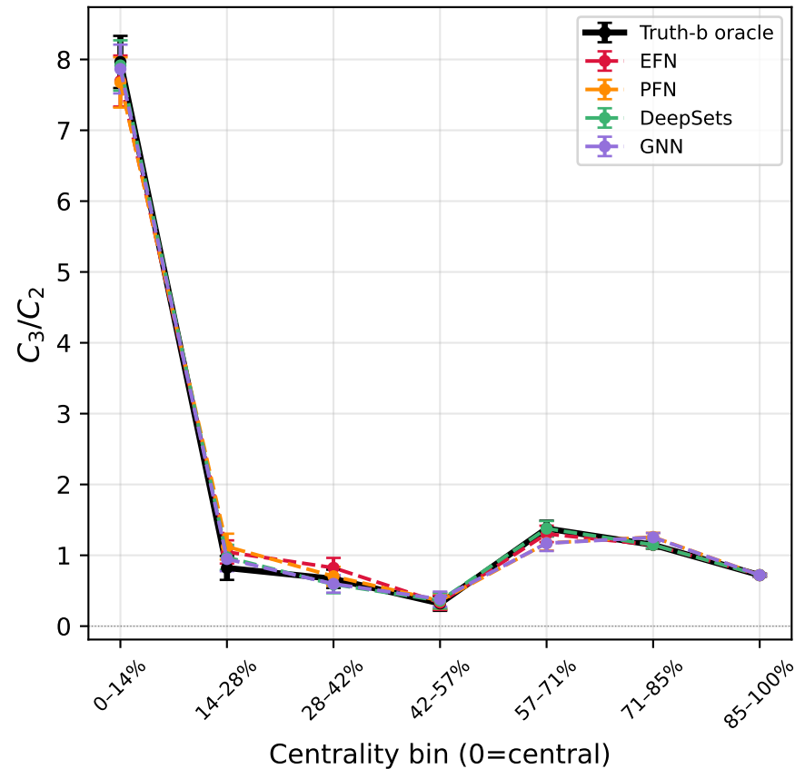
Net-proton cumulant ratios — Au+Au \sqrt{s_{NN}} = 3.9 GeV
