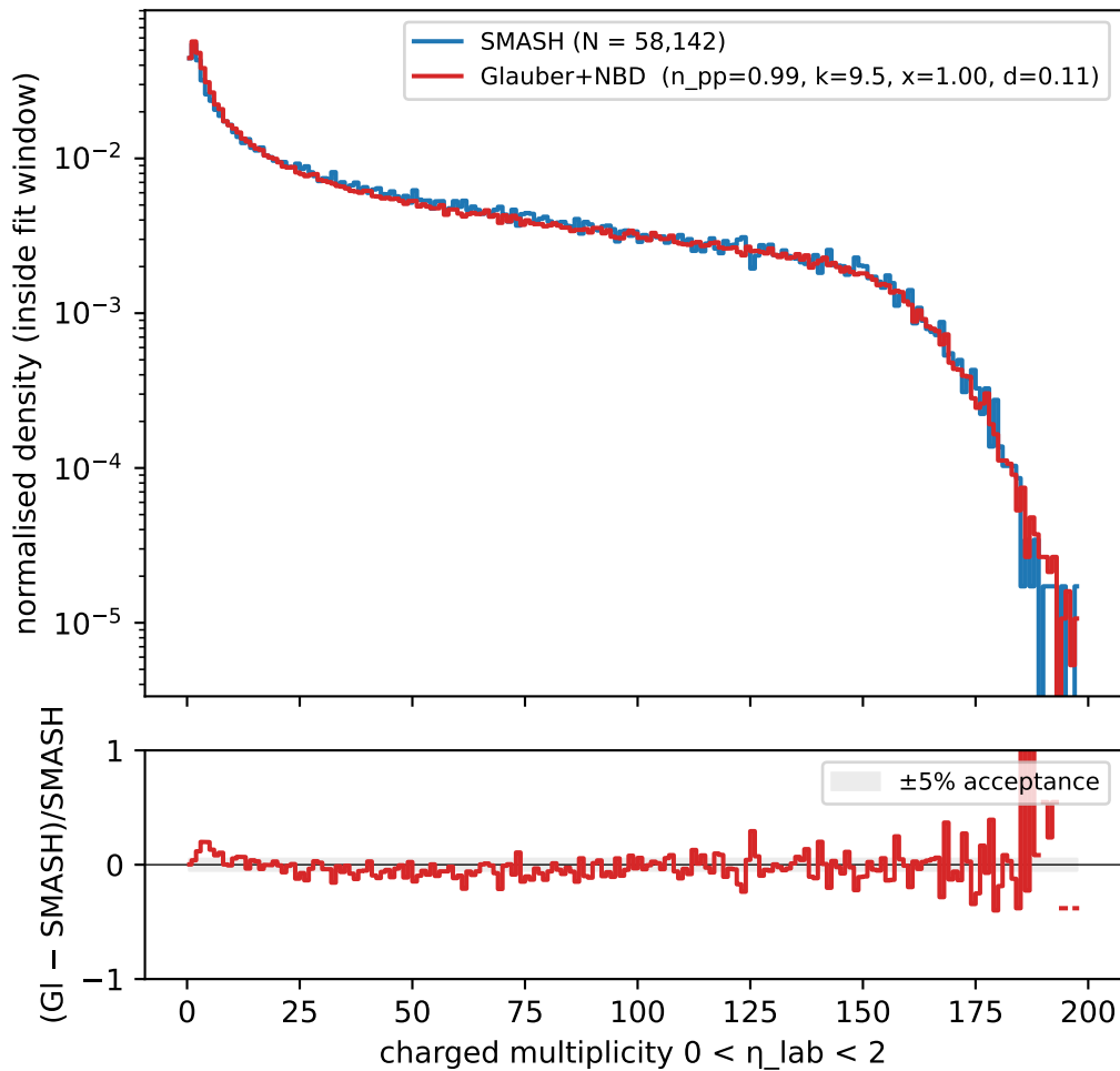
Glauber NBD fit at \sqrt{s_{NN}} = 3.5 GeV \chi^2 = 0.0085
