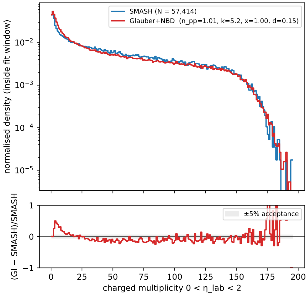
Glauber NBD fit at \sqrt{s_{NN}} = 4.5 GeV \chi^2 = 0.029
