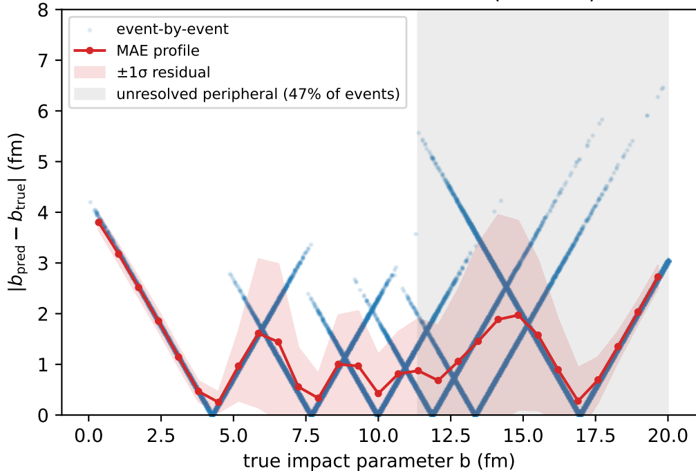
Glauber resolution vs true b (3.2 GeV)
