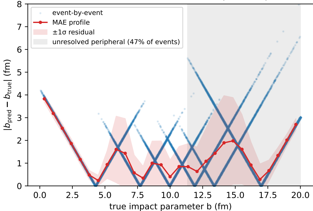
Glauber resolution vs true b (3.5 GeV)
