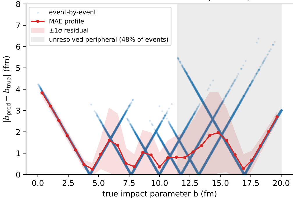
Glauber resolution vs true b (3.9 GeV)
