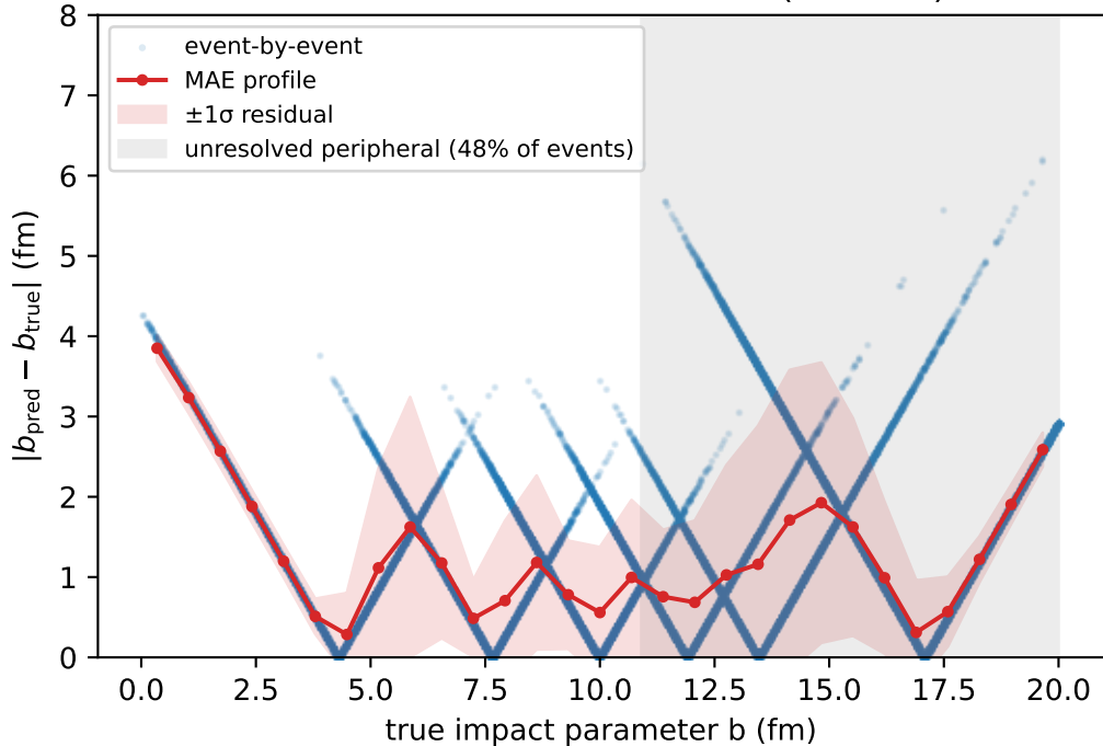
Glauber resolution vs true b (4.5 GeV)
