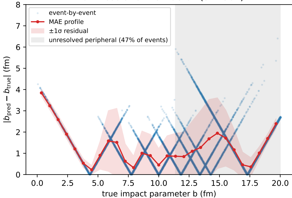
Truth resolution vs true b (3.2 GeV)
