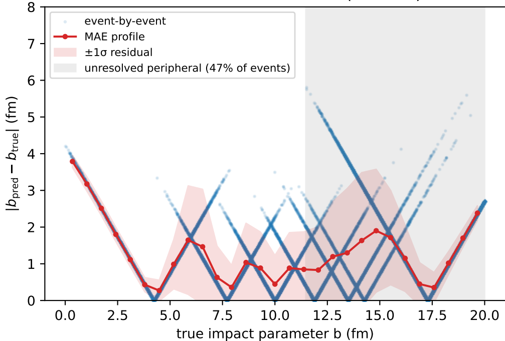
Truth resolution vs true b (3.9 GeV)
