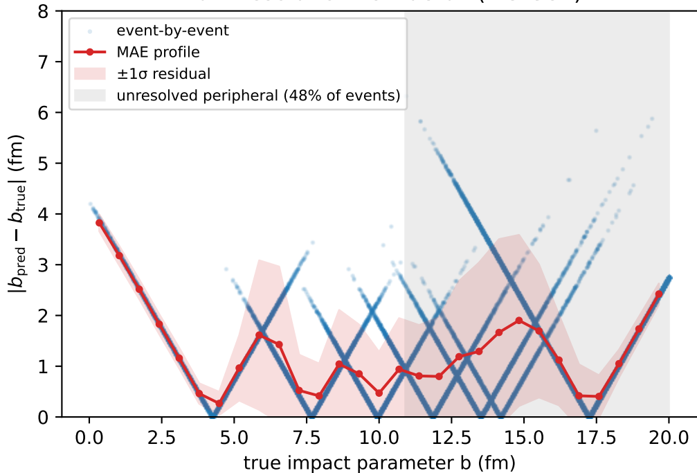
Truth resolution vs true b (4.5 GeV)
