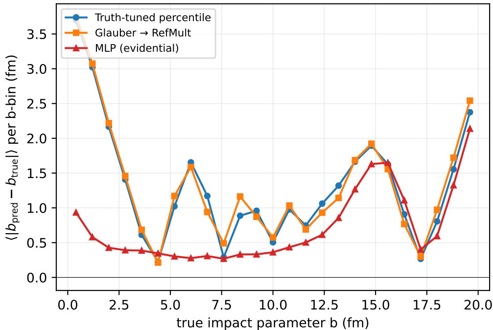
Baseline comparison — 4.5 GeV (N_test = 9,956)
