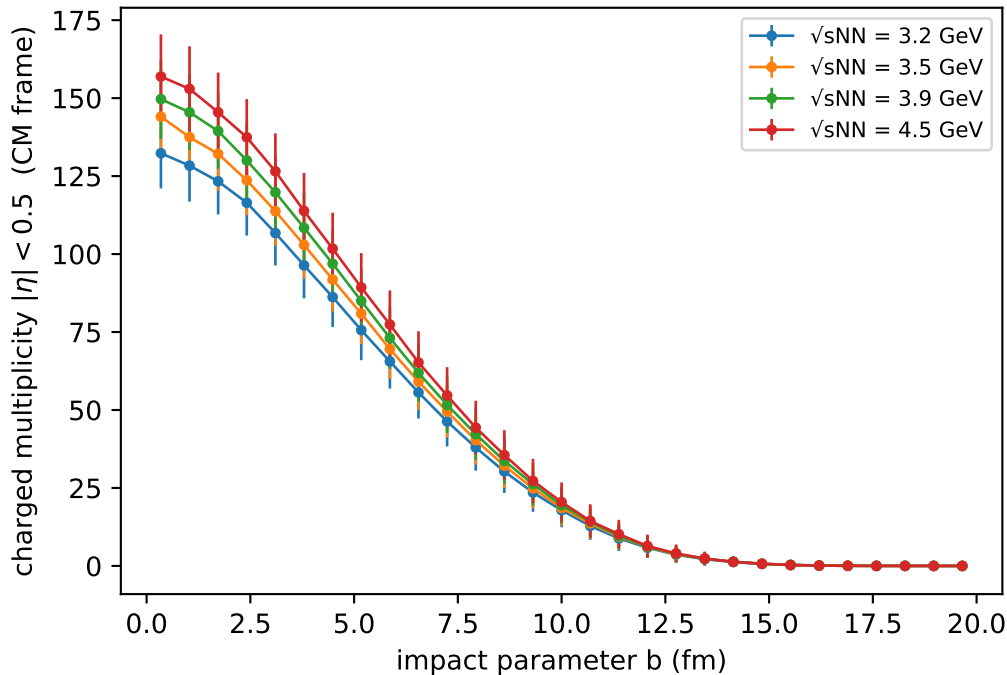
charged mult vs b — all energies
