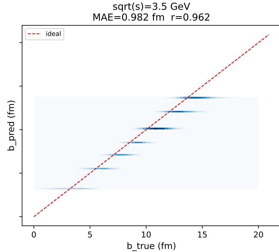
Glauber-NBD -- b_pred vs b_true (test set)
