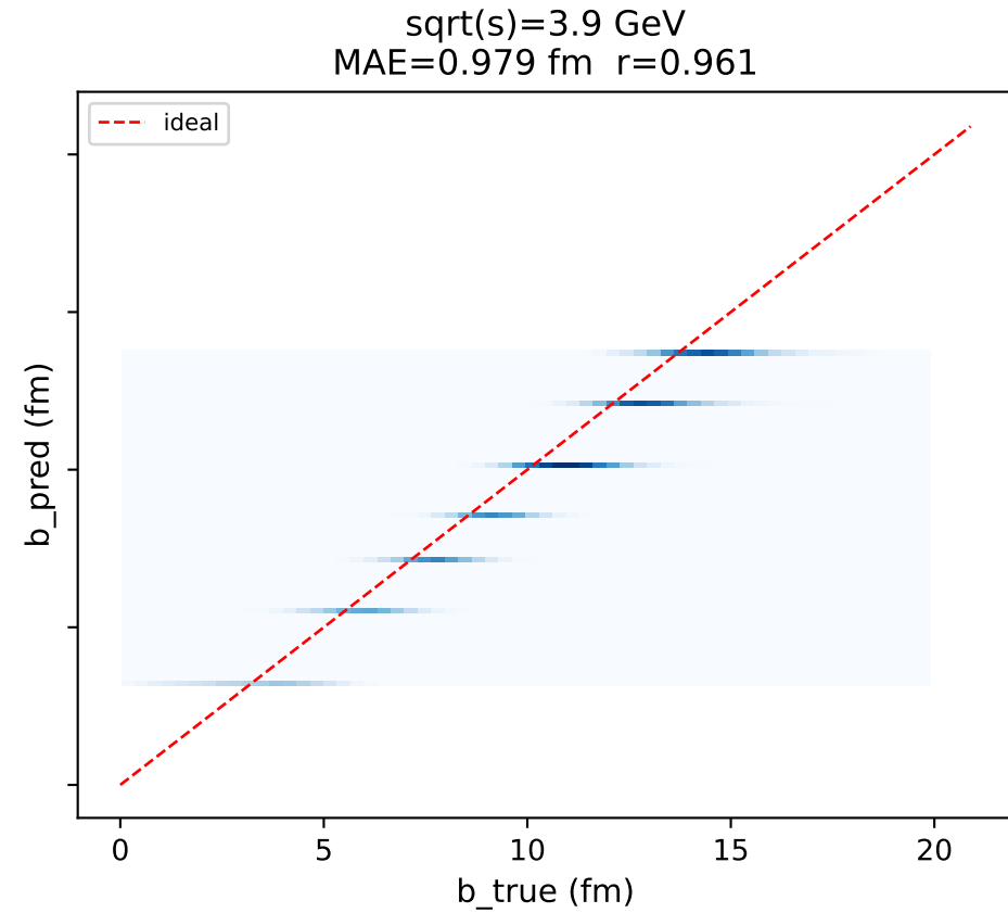
Glauber-NBD -- b_pred vs b_true (test set)
