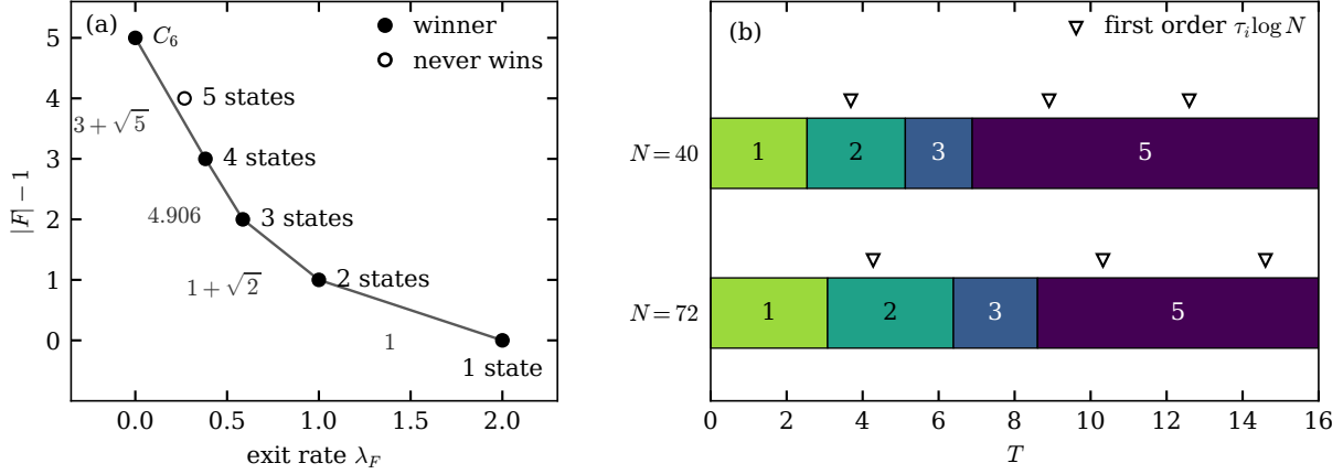
Figure 2: (a) The points (\lambda_F, |F| - 1) of the arcs of the 6-cycle and of C_6 , with the lower-left boundary of their hull. The numbers beside the edges are the switch values \tau_i of Theorem 3.4. The winners (filled) are the arcs of 1 to 4 states and C_6 , and the arc of 5 states (open) never wins. (b) The support size of the exact mode on C_5 with the uniform start, against T , at N = 40 and N = 72 . The mode skips the arc of 4 states. The triangles mark the first-order switch points \tau_i \log N with \tau_i = 1, 1 + \sqrt{2} and 2 + \sqrt{2} (Table 1).
