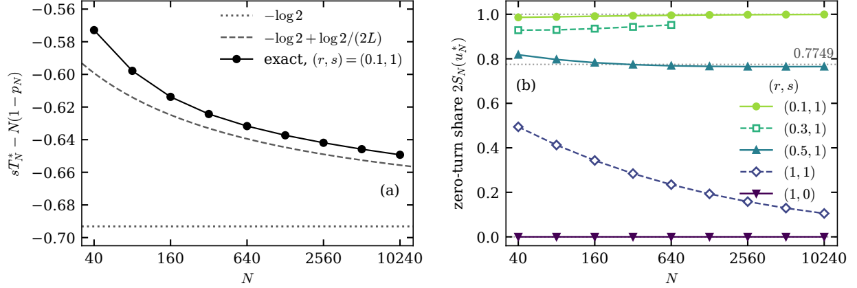
Figure 3: (a) The exact crossing of the planar walk with (r, s) = (0.1, 1) , written as sT_N^* - z_N with z_N = N(1 - p_N) , for N = 40, 80, \dots, 10240 . The dashed curve is -\log 2 + \log 2/(2L) from Theorem 6.4(c), and the dotted line is its limit -\log 2 . (b) The zero-turn share 2S_N(u_N^*) of the origin mass at the crossing. It tends to 1 for s > 2r and to 0 for s < 2r (Theorem 6.3), and by Remark 6.5 (proof omitted) to 2\sqrt{2}/(\sqrt{2} + \sqrt{5}) = 0.7749 at the switch s = 2r . For (r, s) = (1, 0) there are no reversals and the share is 0 for every N . The pair (0.3, 1) was computed up to N = 640 .
