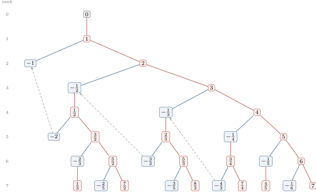
Figure 1: Ranks 0–7 of the tree. Red edges apply f(x) = x + 1 and blue edges apply g(x) = -1/x . Every positive vertex is entered by an f -edge and every negative vertex by a g -edge (Theorem C), and the vertices \leq -1 are leaves. The dashed gray arrows show f applied to the leaves x < -1 : the value x + 1 is not new, and its rank is 3 less than that of x . The numbers on the left are ranks. The rows are Kimberling’s generations [4], with his generation j being rank j - 1 .
