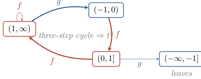
Figure 2: Where the children of each of the 4 classes go (Proposition 5.3). After a g -step, the only way back to the positives is the three-step cycle (1, \infty) \rightarrow (-1, 0) \rightarrow (0, 1] \rightarrow (1, \infty) . This cycle gives the t^3 in the recurrence, and it is the counting version of (gf)^3 = \text{id} (Remark 3.9).
