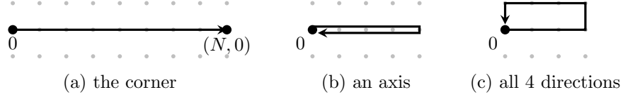
Figure 4: Paths of N = 8 steps. (a) The only path to the corner (N, 0) never switches. A path to the origin either (b) stays on one axis and only reverses, or (c) turns and then uses all 4 directions.
