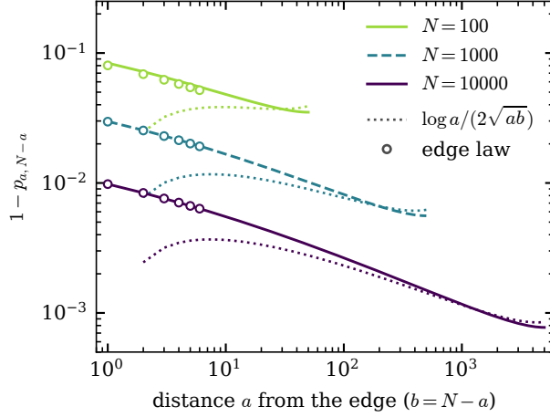
Figure 3: The crossing 1 - p_{a, N-a} of each bin against its distance a from the nearer edge, for N = 100, 1000 and 10^4 . The dotted lines are the leading law (23), and the circles are the edge law (27) for a \leq 6 . The right end of each line is the central crossing 1 - p_N .
