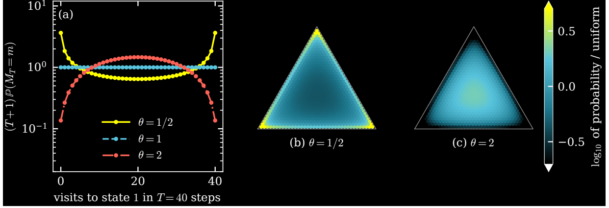
Figure 4: The exact law (10) of the counts of the chain that draws afresh or repeats. (a) Two states and T = 40 , as a multiple of the uniform law. The law is flat at \theta = 1 , the ends are the most likely bins for \theta = \frac{1}{2} , and the center is for \theta = 2 . (b), (c) Three states and T = 36 on the simplex of visit fractions. Each cell is one bin, colored by its probability relative to the uniform law. For \theta = \frac{1}{2} a corner is 9.6 times as likely as under the uniform law and the center 0.43 times. For \theta = 2 the numbers are 0.035 and 2.1.
