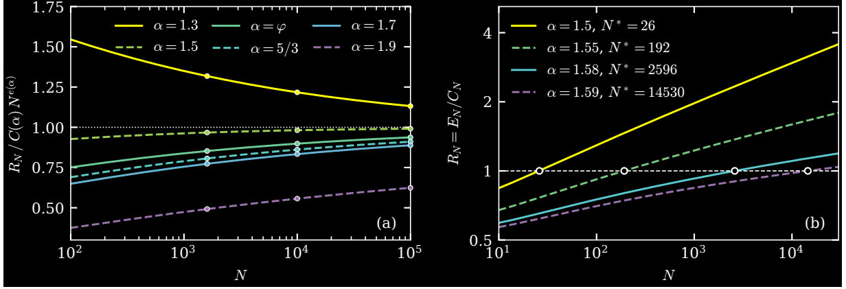
Figure 3: Alternating runs with a stationary start. (a) R_N / (C(\alpha) N^{e(\alpha)}) for even N from 100 to 10^5 , with the entries of Table 2 as dots. (b) R_N for \alpha = 1.5, 1.55, 1.58, 1.59 below \varphi . Each curve crosses 1 once on 10 \leq N \leq 3 \cdot 10^4 , at N^*(\alpha) (circles).
