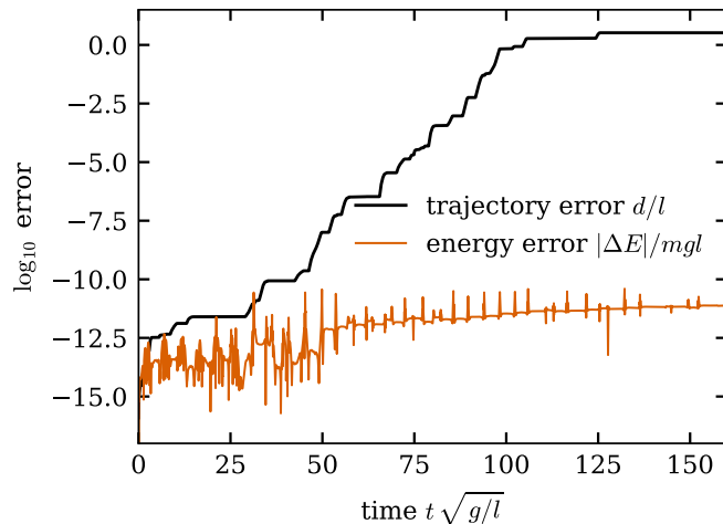
FIG. 6. Error in the position of the lower bob and error in the energy for one run in double precision ( p = 53 ) with h = 2^{-10} . The energy error stays below 10^{-10} throughout, while the trajectory is lost near t = 92 .
