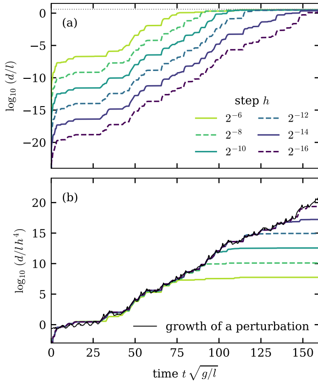
FIG. 2. (a) Running maximum of the separation d of the lower bob from that of the reference run ( h = 2^{-18} ) for six values of the step, in 237-bit arithmetic. The dotted line marks the largest possible separation, 4l . (b) The same curves multiplied by h^{-4} collapse. The thin black line is the separation, in the four-dimensional state space, of two runs whose initial conditions differ by 2^{-170} , shifted vertically.
