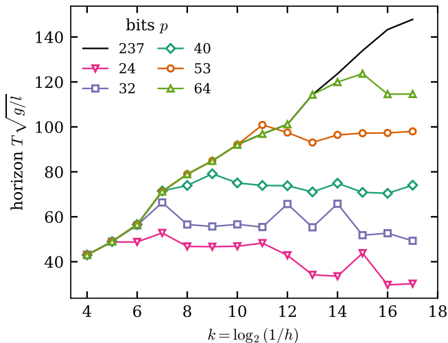
FIG. 3. Horizon against step for five working precisions, with the 237-bit result of Fig. 2(a) for comparison. For each precision there is a step beyond which further refinement does not help.
