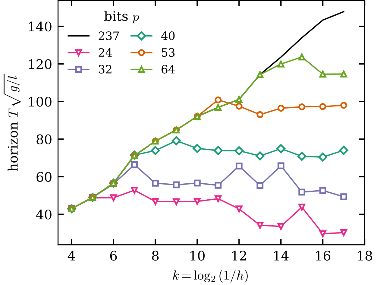
FIG. 4. Horizon against step for five working precisions, with the 237-bit result of Fig. 2(a) for comparison. For each precision there is a step beyond which further refinement does not help.
