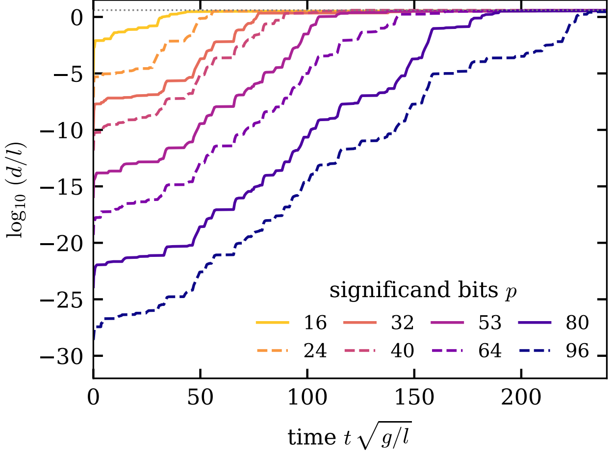
FIG. 3. Separation from the 237-bit run at the same step, h = 2^{-12} , for eight significantand widths p . Truncation error is common to each pair of runs and cancels, so the curves show the effect of roundoff alone.
