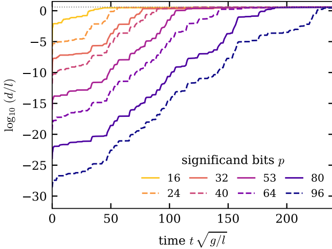
FIG. 3. Separation from the 237-bit run at the same step, h = 2^{-12} , for eight significant widths p . Truncation error is common to each pair of runs and cancels, so the curves show the effect of roundoff alone.
