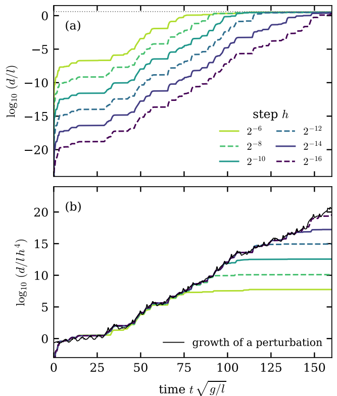
FIG. 1. (a) Separation d of the lower bob from that of the reference run ( h = 2^{-18} ) for six values of the step, in 237-bit arithmetic; the running maximum is shown. The dotted line marks the largest possible separation, 4l . (b) The same curves multiplied by h^{-4} collapse. The thin black line is the separation of two runs whose initial conditions differ by 2^{-170} , shifted vertically.
