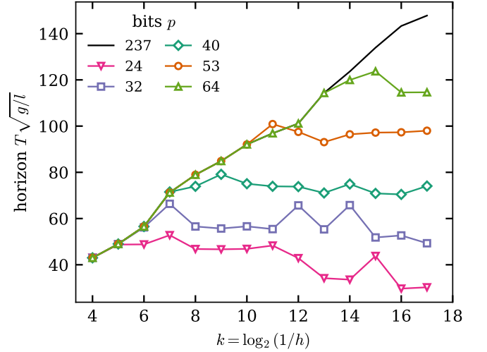
FIG. 5. Horizon against step for five working precisions, with the 237-bit result of Fig. 3(a) for comparison. For each precision there is a step beyond which further refinement does not help.
