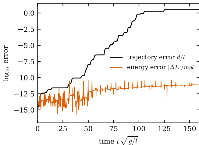
FIG. 6. Error in the position of the lower bob and error in the energy for one run in double precision ( p = 53 ) with h = 2^{-10} . Energy remains conserved to better than a part in 10^{10} throughout, while the trajectory is lost near t = 92 .
