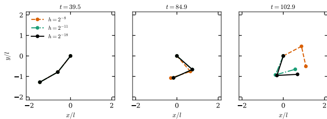
FIG. 1. Three double pendulums released from the same state and integrated with the same 237-bit arithmetic, differing only in the step h . The run with h = 2^{-8} leaves the others near t = 79 , and the run with h = 2^{-11} near t = 97 . Times are in units of \sqrt{l/g} .
