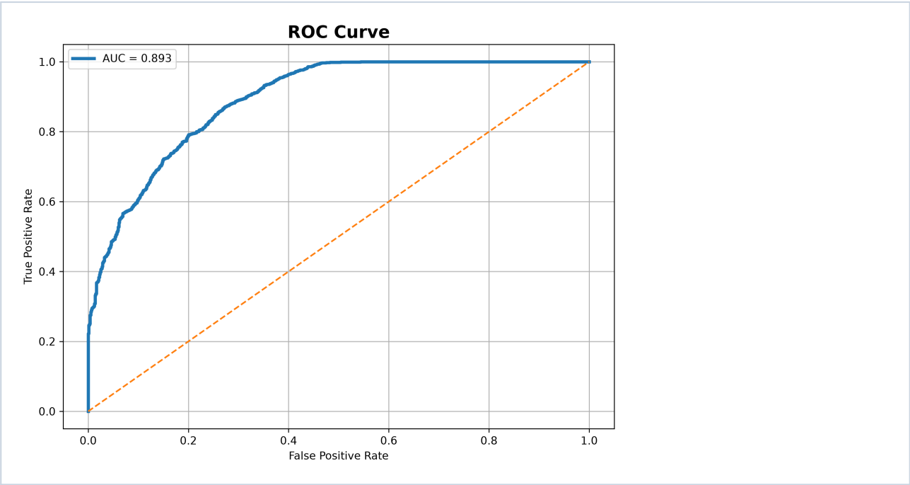
Model discrimination performance across threshold settings.
