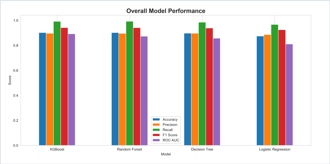
Consolidated overview of model diagnostics and performance.
