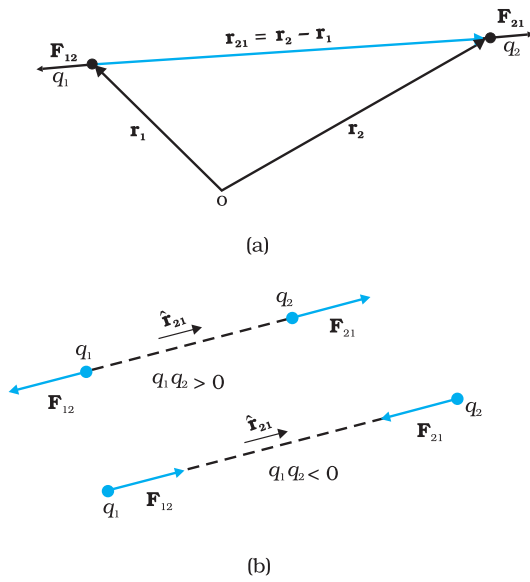
FIGURE 1.3 (a) Geometry and (b) Forces between charges.
