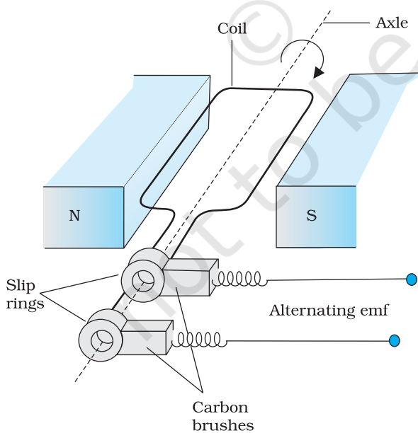
FIGURE 6.13 AC Generator
