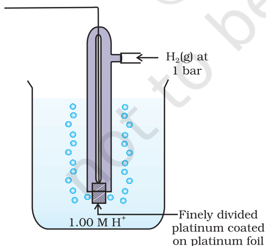
Fig. 2.3: Standard Hydrogen Electrode (SHE).
