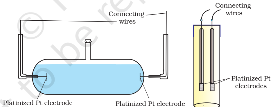
Fig. 2.4 Two different types of conductivity cells.
