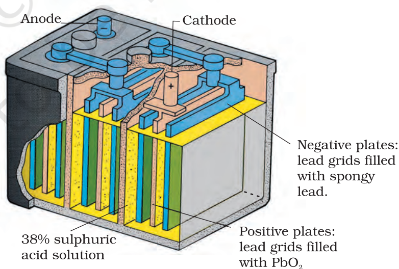
Fig. 2.10: The Lead storage battery.
