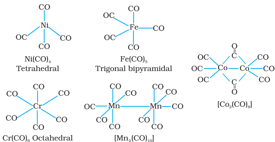
Fig. 5.13 Structures of some representative homoleptic metal carbonyls.
