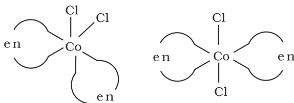
Fig. 5.4: Geometrical isomers (cis and trans) of [\text{CoCl}_2(\text{en})_2]
