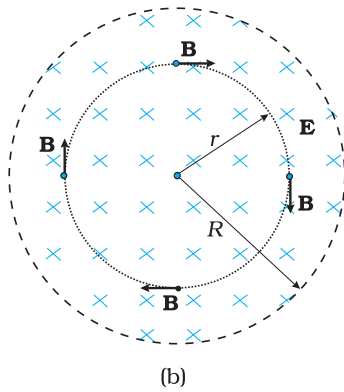
FIGURE 8.2 (a) The electric and magnetic fields E and B between the capacitor plates, at the point M. (b) A cross sectional view of Fig. (a).
