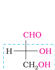
D- (+) - Glyceraldehyde
