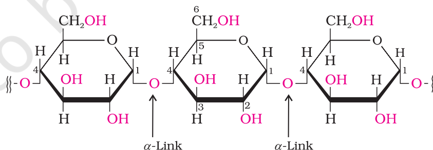
Amylose
