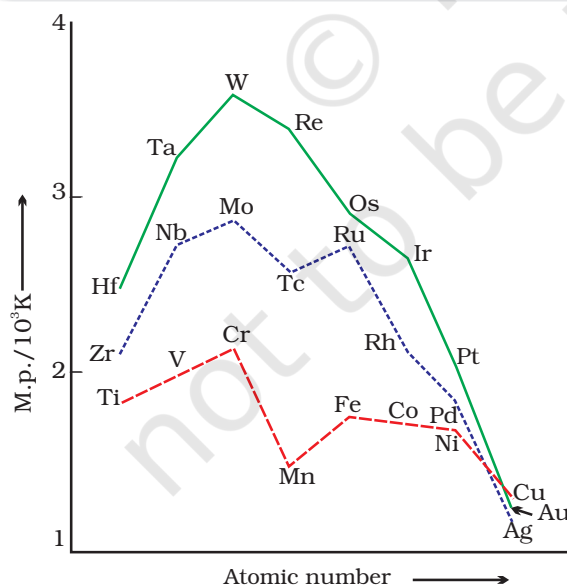
Fig. 4.1: Trends in melting points of transition elements
