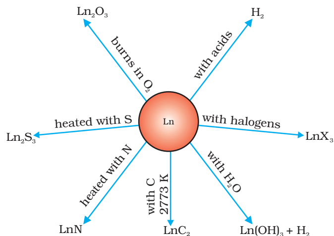
Fig 4.7: Chemical reactions of the lanthanoids.
