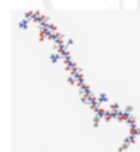
MOLECULAR STRUCTURE
