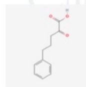
MOLECULAR STRUCTURE
