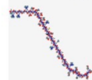
MOLECULAR STRUCTURE
