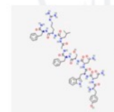
MOLECULAR STRUCTURE
