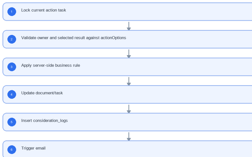
LLDD BE - API Document Workflow Actions
