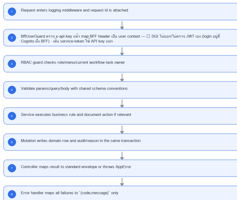
LLDD BE - API Common Contracts
