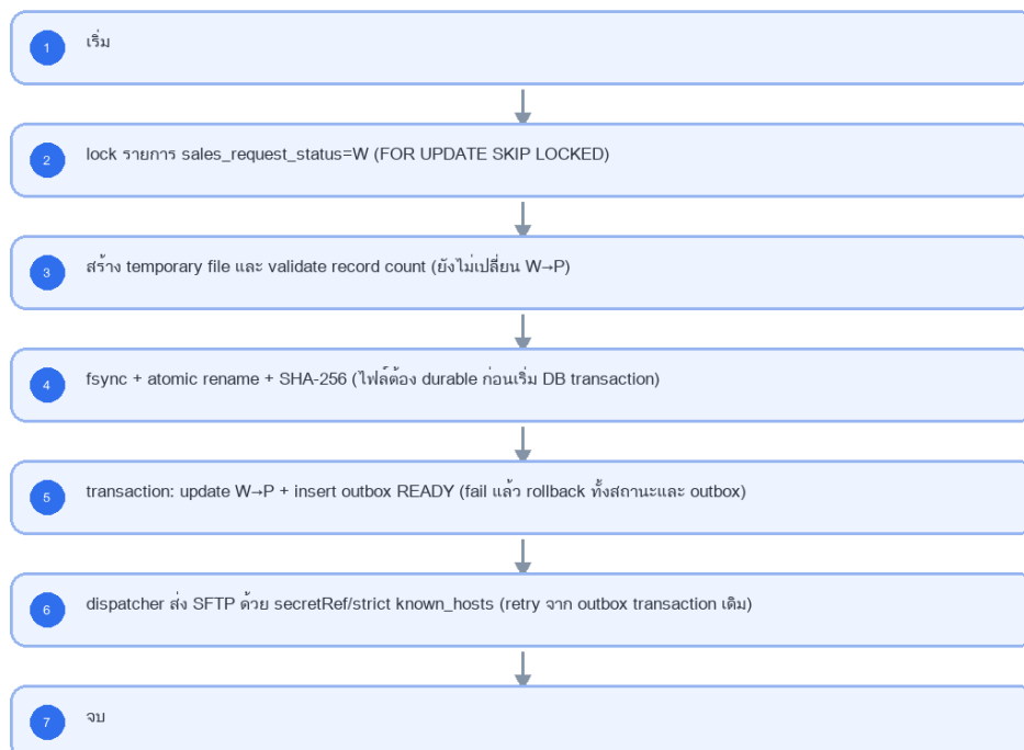
LLDD BE - Job 4 PrepareImpactStoreToIAS
