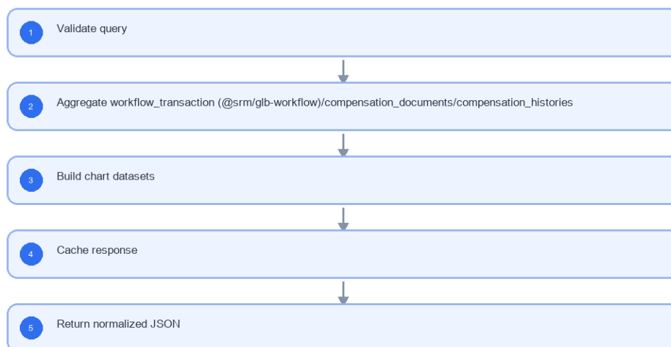
LLDD BE - API Dashboard Summary
