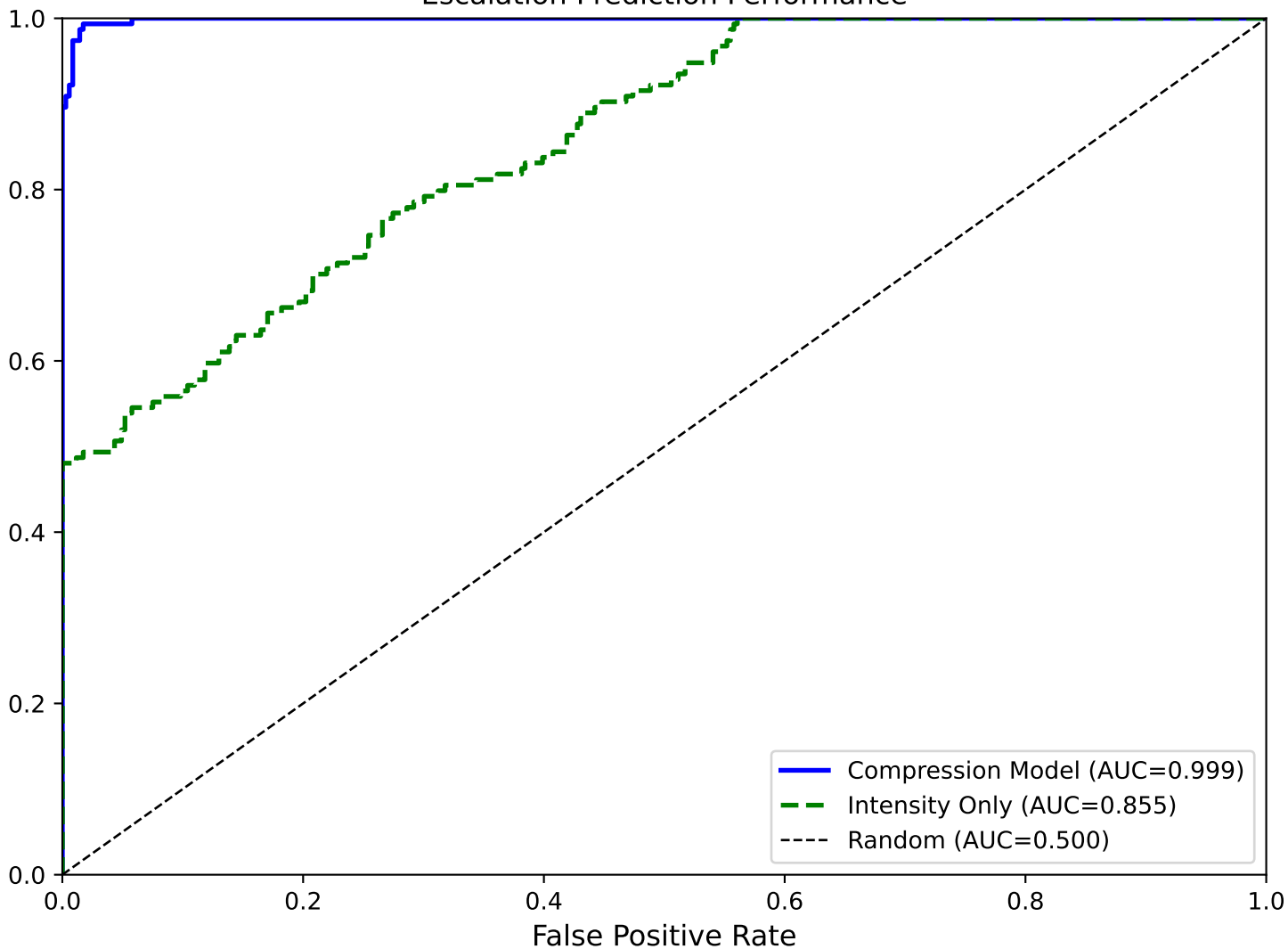
Escalation Prediction Performance
