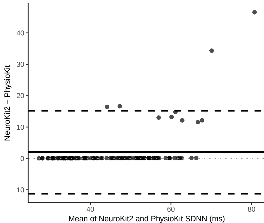
Bland-Altman Plot: SDNN (ms)
