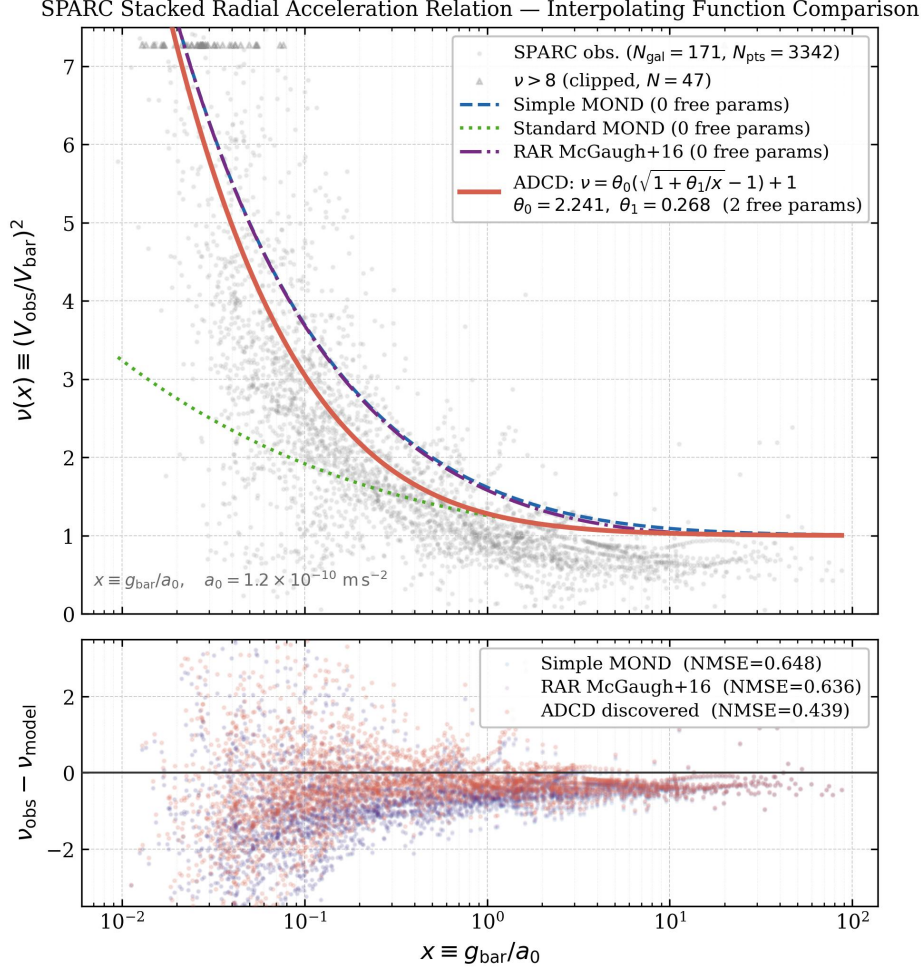
Figure 7: SPARC stacked radial acceleration relation. Upper: observed \nu(x) (grey) against the four interpolating functions. The ADCD-discovered 2-parameter curve (red) tracks the data more tightly than Simple/Standard MOND and the McGaugh+16 RAR form. Lower: residuals \nu_{\text{obs}} - \nu_{\text{model}} .
