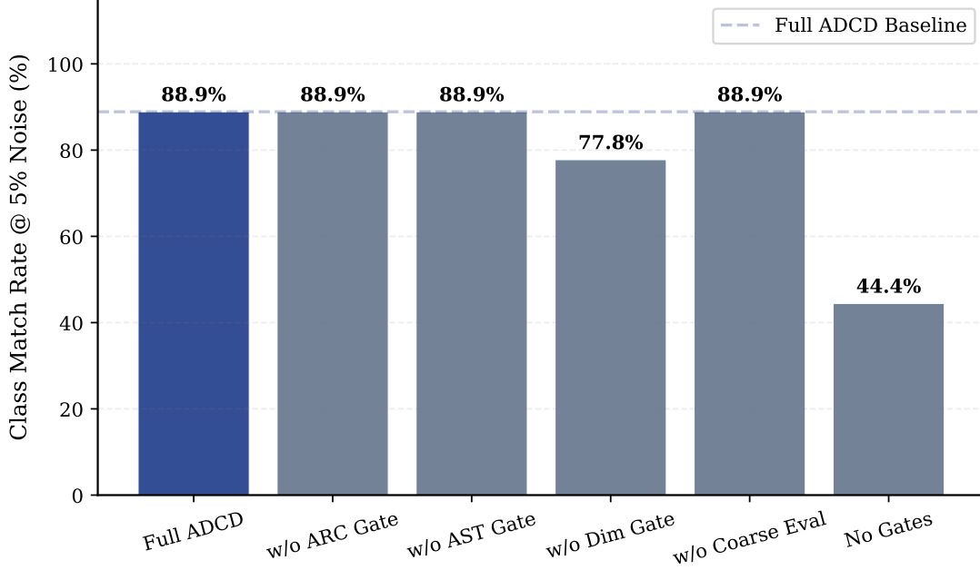
Figure 6: Ablation study at 5% observational noise. Each bar disables one gate. Removing the ARC, AST, or Coarse-Eval gate individually leaves structural accuracy unchanged (8/9). Removing the dimensional gate alone reduces accuracy by 11.1 pp (8/9 to 7/9). Only removing all gates simultaneously causes a larger collapse, dropping performance by \Delta = 44.5 percentage points (from 8/9 to 4/9), confirming that the gates reinforce each other as a collective physical consistency filter. Note: the “Without BIC Reranking” condition is described in Section 6 but excluded from this figure as it requires the full gate pipeline to isolate BIC’s contribution.
