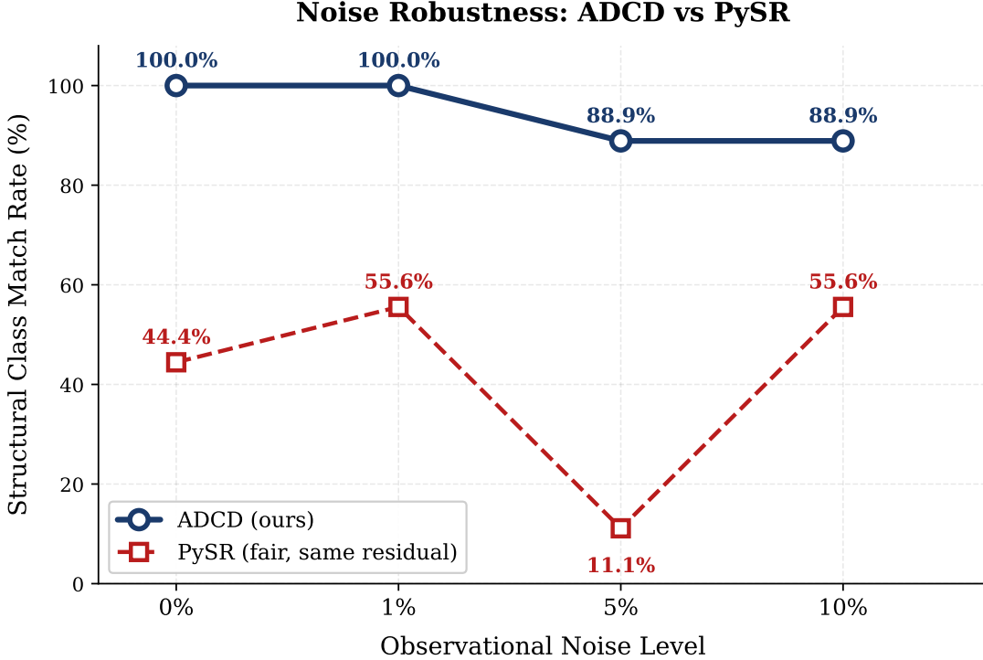
Figure 3: Structural class match rate as a function of observational noise level. ADCD (Mock Proposer, seed=42) maintains 88.9% structural accuracy at 5% noise due to physics-constrained gate filtering. PySR (fair profile, unconstrained SR on the same residual) exhibits a non-monotonic noise–accuracy profile (44.4%→55.6%→11.1%→55.6%), reflecting overfitting instabilities absent from physics-gated search.
