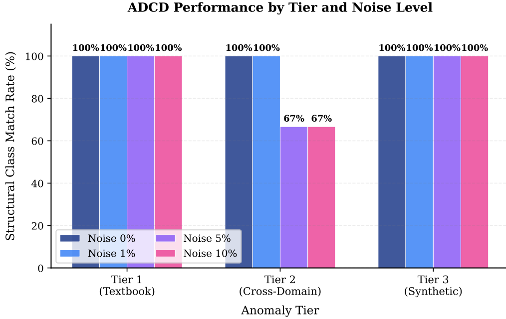
Figure 5: Structural class match rate grouped by anomaly tier and noise level. The synthetic tier achieves 100% recovery at all noise levels; degradation is localized to the Screened Coulomb scenario at \geq 5\% noise.
