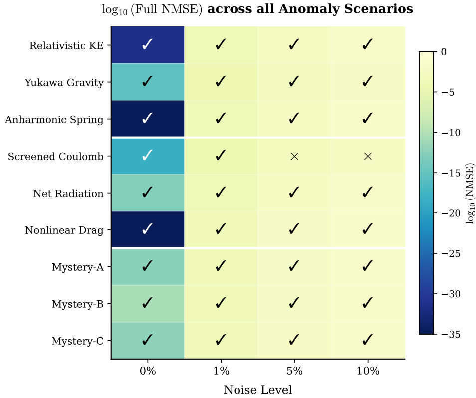
Figure 4: Log-scale NMSE heatmap across all 9 anomaly scenarios and 4 noise levels. Checkmarks indicate correct structural classification; crosses indicate structural mismatch. White lines separate tiers.
