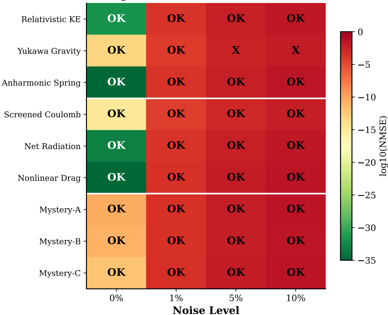
log10(Full NMSE) - All Scenarios
