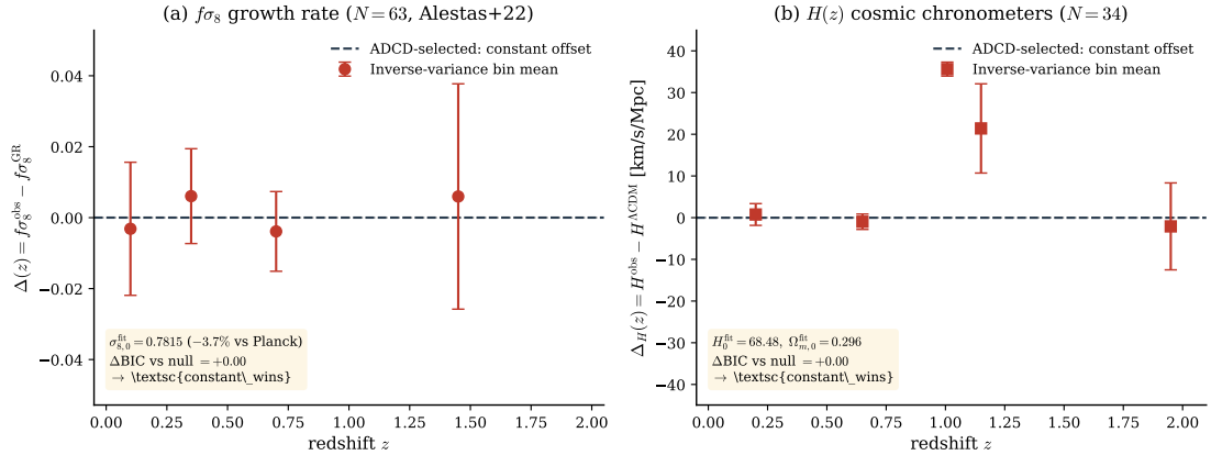
Figure 7: Cosmological-probe residuals and the CONSTANT_WINS verdict. (a) f\sigma_8 residual \Delta(z) = f\sigma_8^{\text{obs}} - f\sigma_8^{\text{GR}} (63 points, Alestas+22); the GR baseline has \sigma_{8,0} free. Inverse-variance bin means (red) are consistent with zero across all redshifts ( |\text{pull}| \leq 0.5\sigma ), and the ADCD-selected model is the 1-parameter constant offset (dashed). (b) Same for H(z) (34 cosmic-chronometer points); the best candidate is again the constant offset. In both observables no z -dependent functional form beats a pure amplitude rescaling by \Delta\text{BIC} < -10 .
